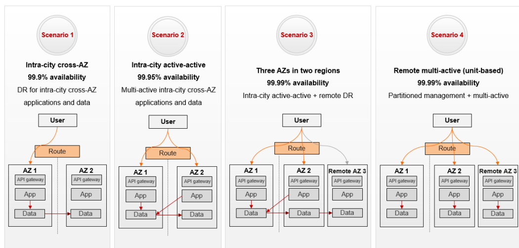
Figure 2-1 MAS application scenarios
